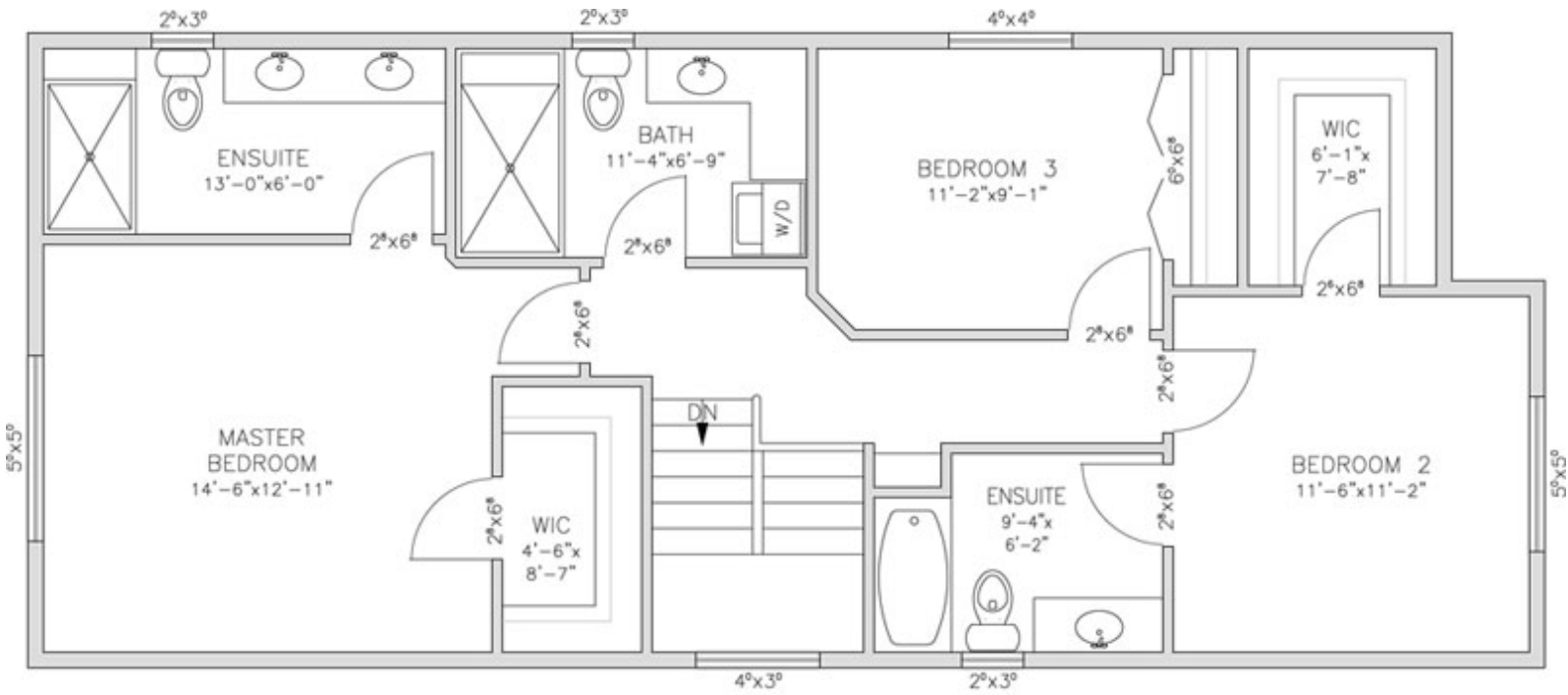
UPPER FLOOR PLAN 980 SQ FT
