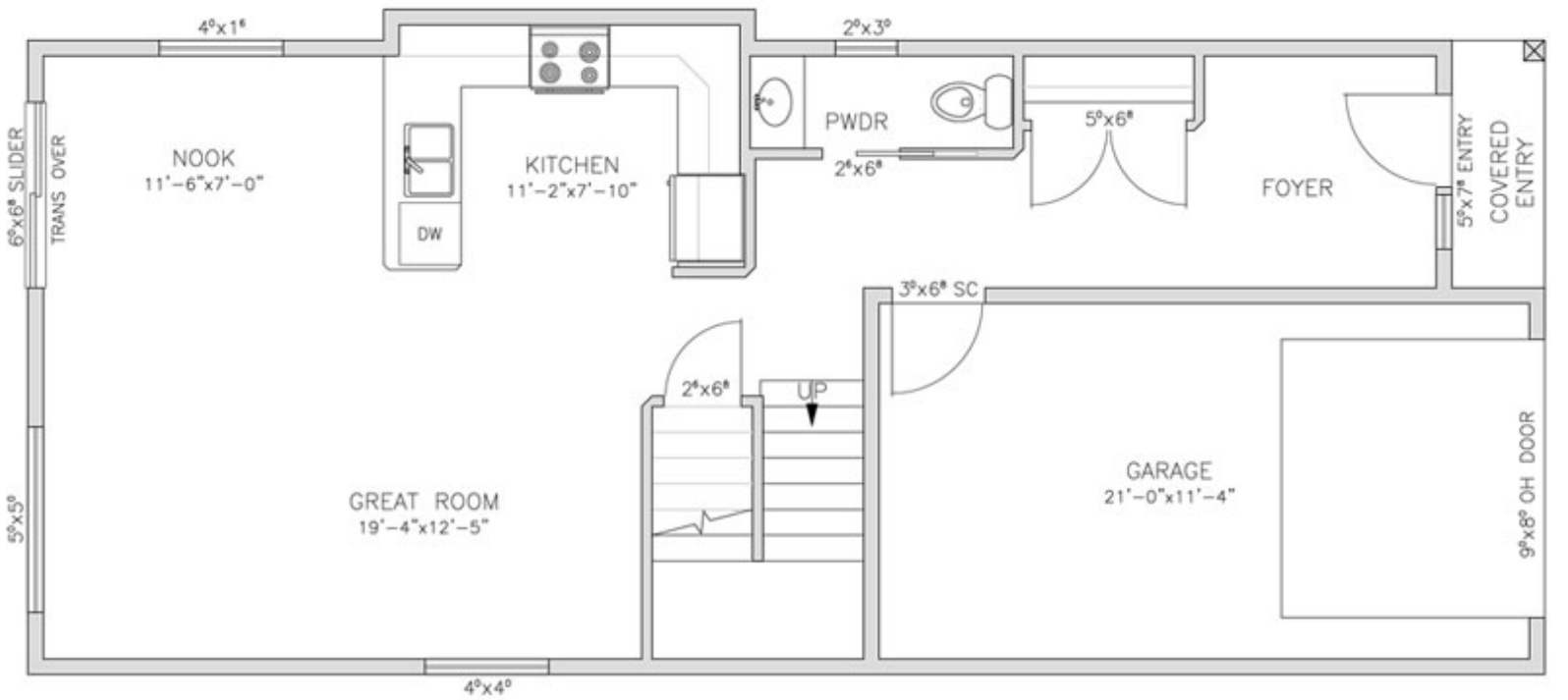
MAIN FLOOR PLAN 733 SQ FT
