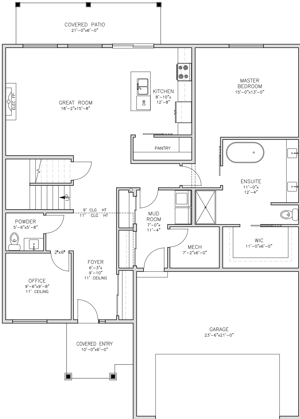
MAIN FLOOR PLAN 1582 SQ FT
