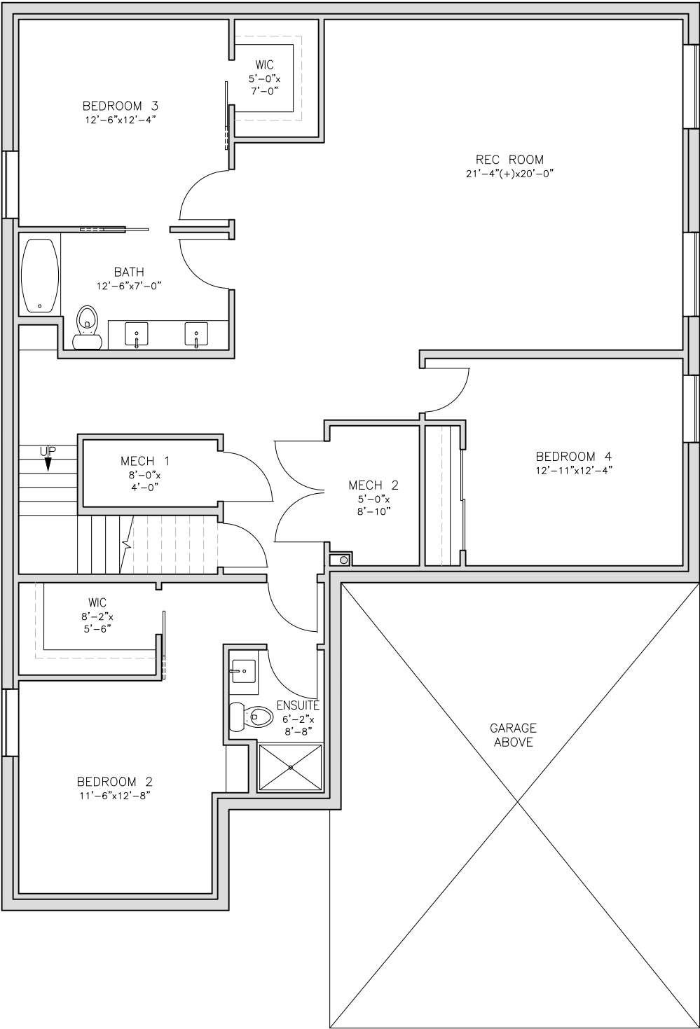
LOWER FLOOR PLAN 1783 SQ FT
